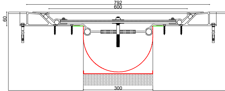
■ Z-5000 W-300W792 JW : 300 H: 60 S: 792 BW: 850 M: 500
