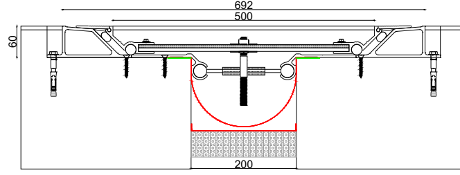
■ Z-5000 W-200W692 JW : 200 H: 60 S: 692 BW: 750 M: 400
