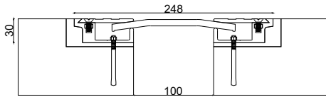
■ Z-6000-100W248 JW : 100 H: 30 S: 248 M: 80
