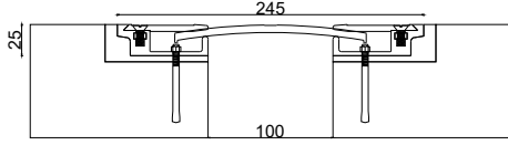
■ Z-6000-100W245 JW : 100 H: 25 S: 245 M: 80
