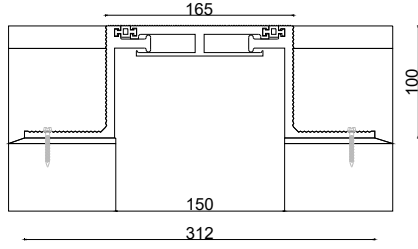
■ Z-1520 -150W165 JW :150 H: 100 S: 165 BW: 312 M: 15
