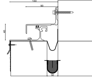
RK 2001-30W90 JW :30 H:40 S:90 BW:133 M:30
