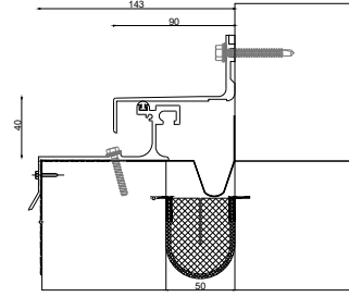
RK 2001-50W90 JW :50 H:40 S:90 BW:143 M:50
