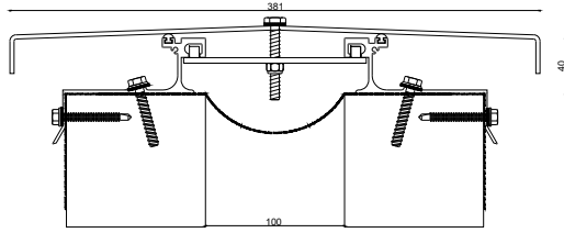
R 2001-100W381 JW :100 H:40 S:381 BW:381 M:100
