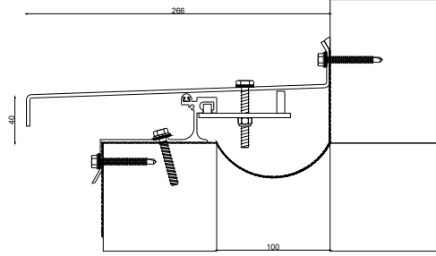
RK 2001-100W266 JW :100 H:40 S:266 BW:266 M:100
