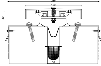
R 2001-30W150 JW :30 H:40 S:150 BW:235 M:30
